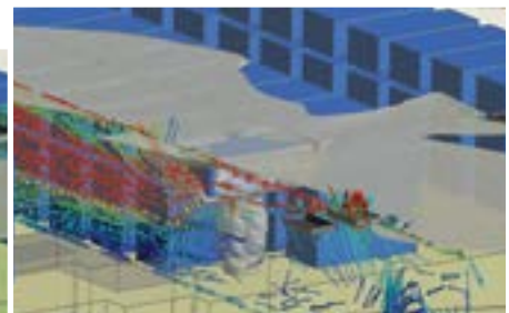
Images above showing a transient combustion model of a car stacker system.
