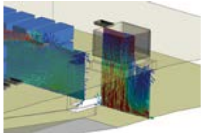
Images above showing how an engineering approach improves a design - by removing the supply in the ceiling, smoke is no longer dragged to low level giving better visibility with the car park.
