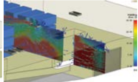
Images above showing how an engineering approach improves a design - by removing the supply in the ceiling, smoke is no longer dragged to low level giving better visibility with the car park.
